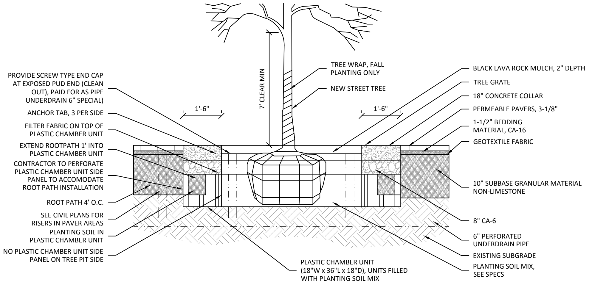
TREE PIT ROOT SECTION WITH PLASTIC CHAMBER UNIT
